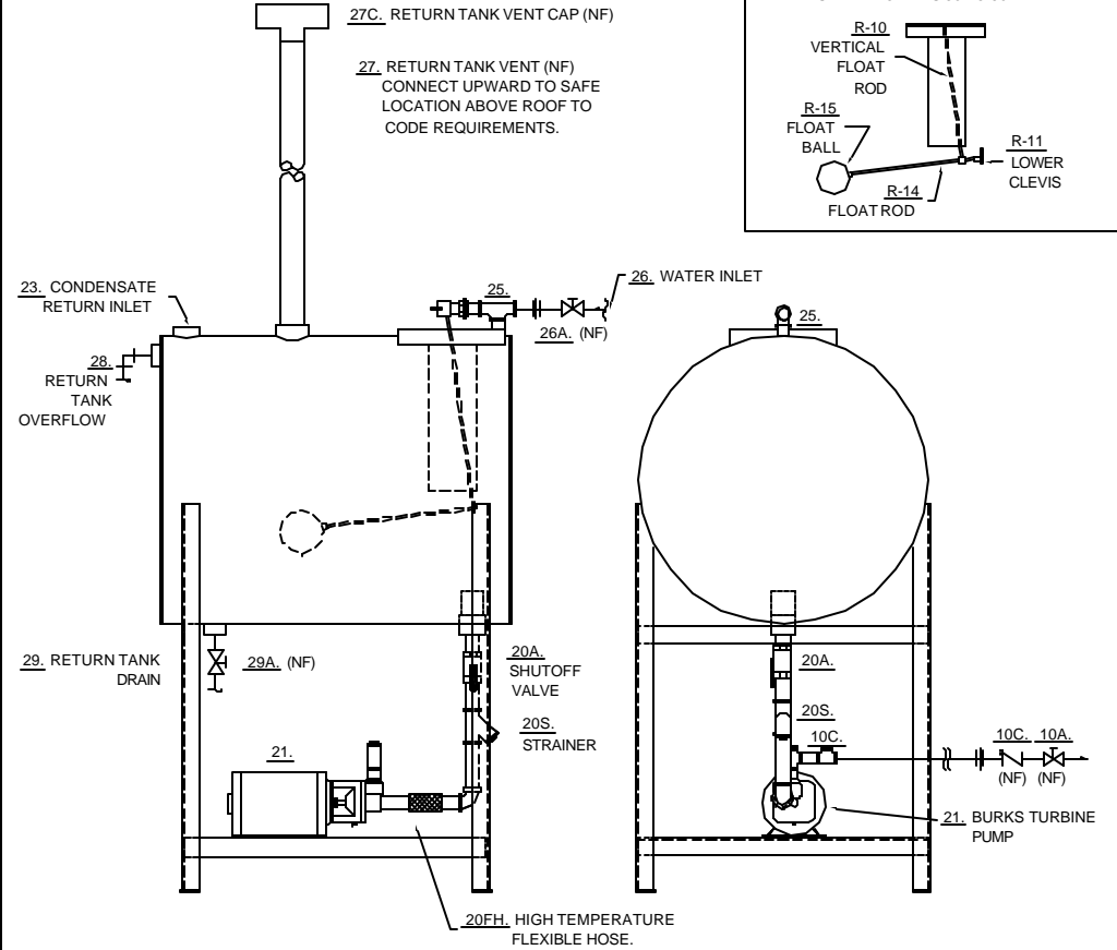
RETURN SYSTEMS R-5 TO R-6 30 TO 50 H.P. BOILERS MODEL WRH ROUND TANKS
