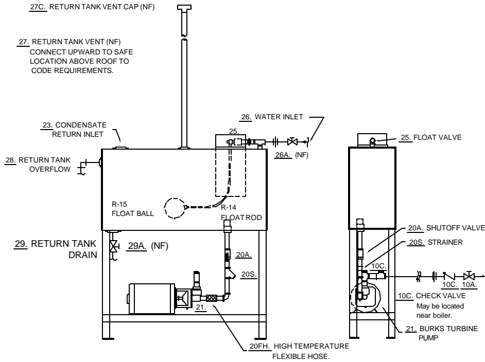
RETURN SYSTEMS R-1 TO R-4 1-1/2 TO 25 H.P. BOILERS MODEL ORR RECTANGULAR TANKS
