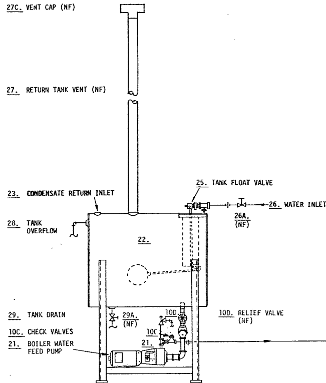
22. WATER MAKE-UP AND CONDENSATE RETURN TANK (See separate Return System Installation Sheet)
