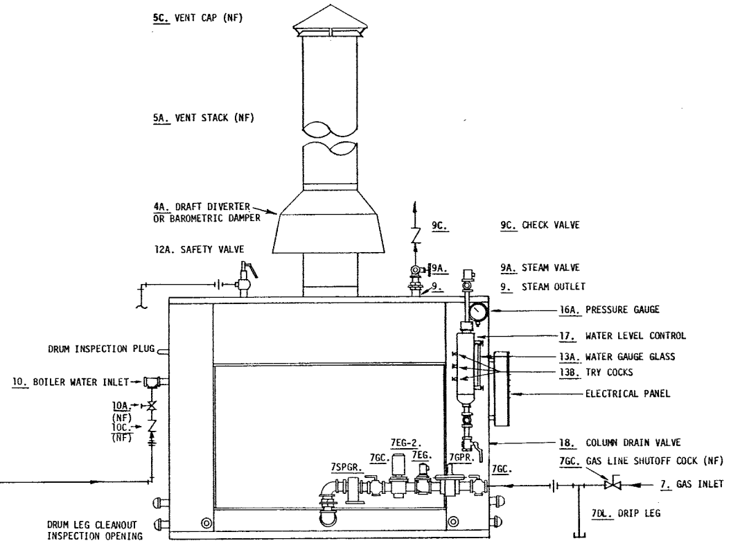
PARKER INDUSTRIAL STEAM BOILER GAS FIRED - FRONT VIEW (See separate Installation Drawing for Blowdown and Drain Lines)
